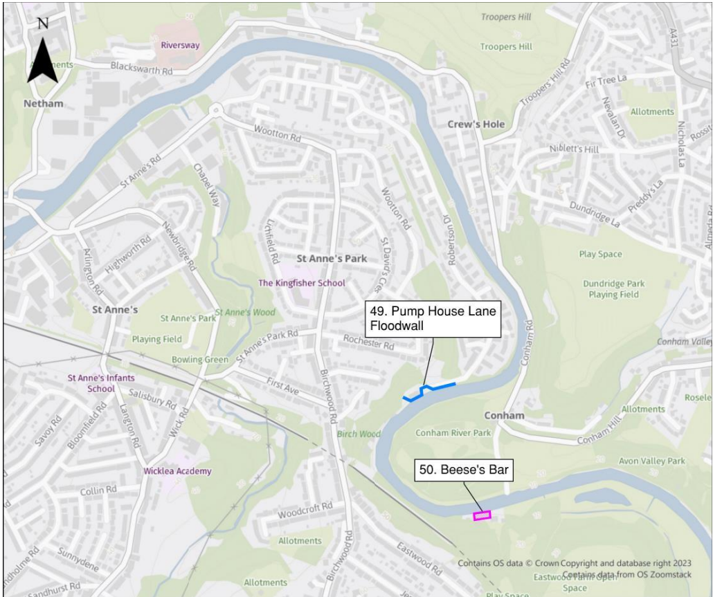
Figure 22 – Upstream of St Anne's (blue and pink lines delineate between defence sections)
