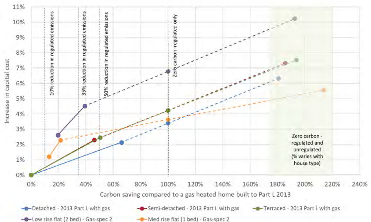
Figure 4.6 Cost and performance of options to achieve policy option 3 with gas heating
