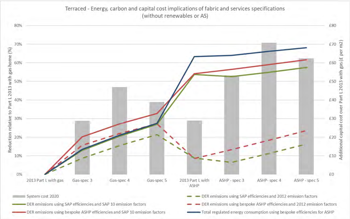
Figure D.3 Cost uplift and energy and carbon savings with different modelling assumptions – terraced house
